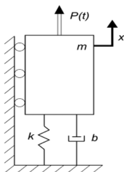
Fig. 2. Calculation model
