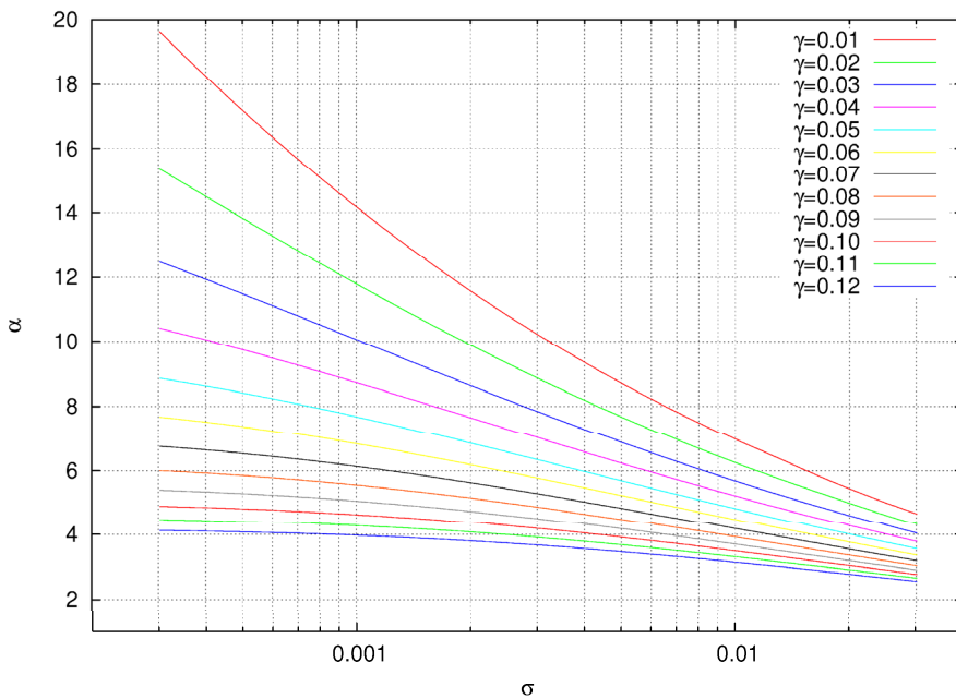
Fig. 5. Nomogram (Cieplik, 2009a) for the determination of maximal amplitudes at the free coasting of the symmetric machine and of the machine of a linear vibration trajectory.
